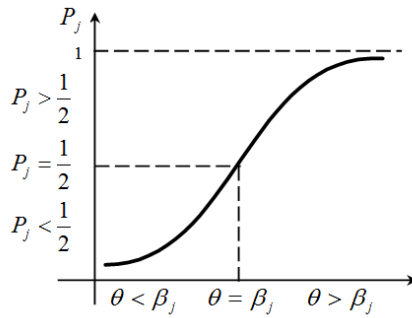
Figure 6. The graph of P_j=F(\theta) (response curve of item)
