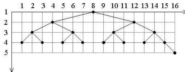
Figure 4. Bisection strategies for 16 tasks scheme
