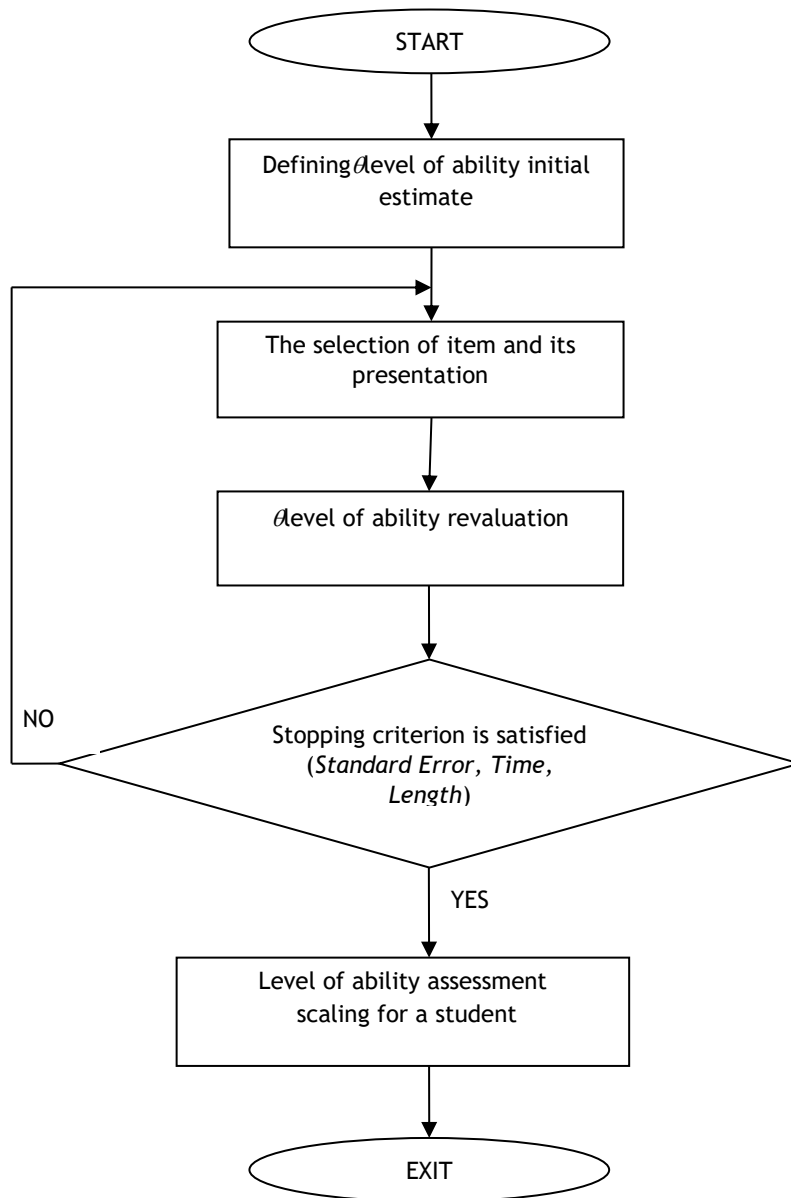
Figure 7. Flexible strategy algorithm of adaptive measurement
