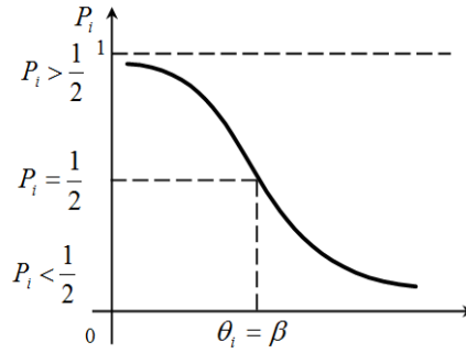
Figure 5. The graph of P_i=f(\beta) (individual curve of a testee)
